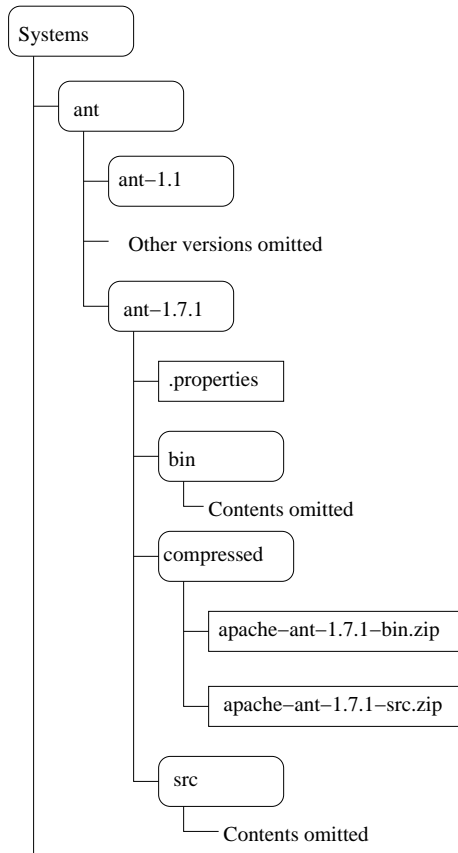
Figure 1. Organisation of Qualitas Corpus.
